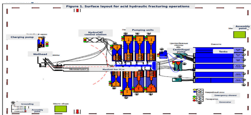
Figure 1. Location of equipment for acid hydraulic fracturing.
